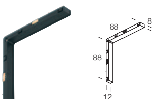
track MICRO P L-joint for ceiling/wall mount
